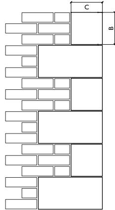
Plain Quoin Q 1
