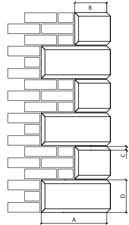
Chamfered Quoin Q 2
